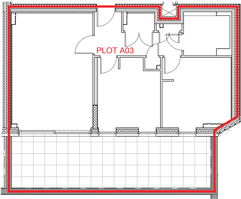
Plot A03 Plan (Ground Floor) 1:100
