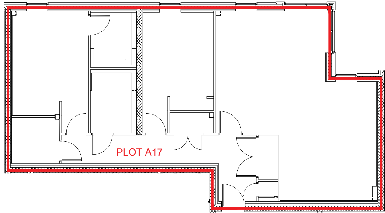
Plot A17 Plan (Second Floor) 1:100
