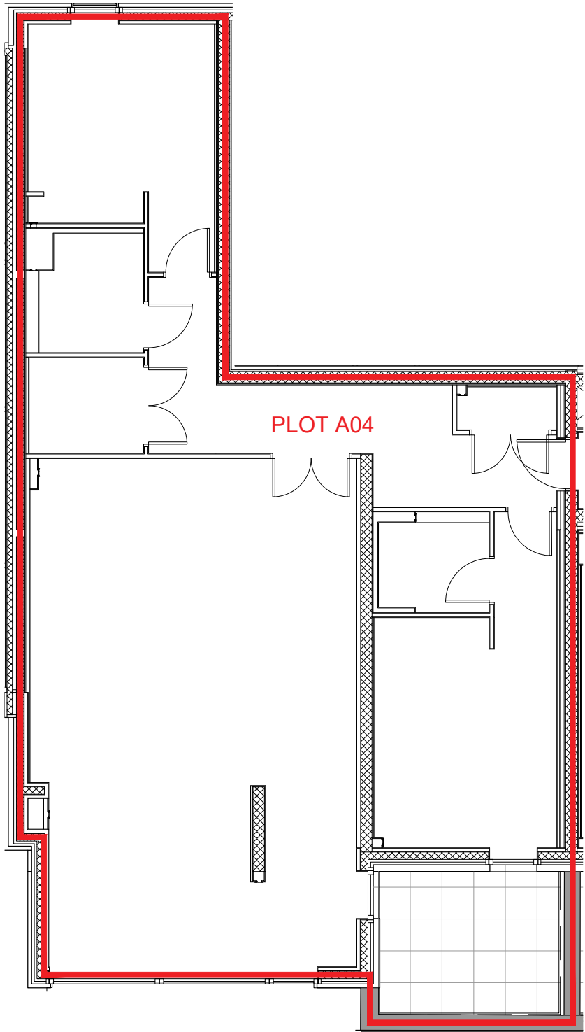
Plot A04 Plan (Ground Floor) 1:100
