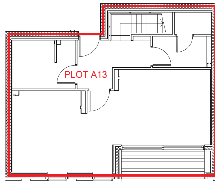
Plot A13 Plan (Second Floor) 1:100
