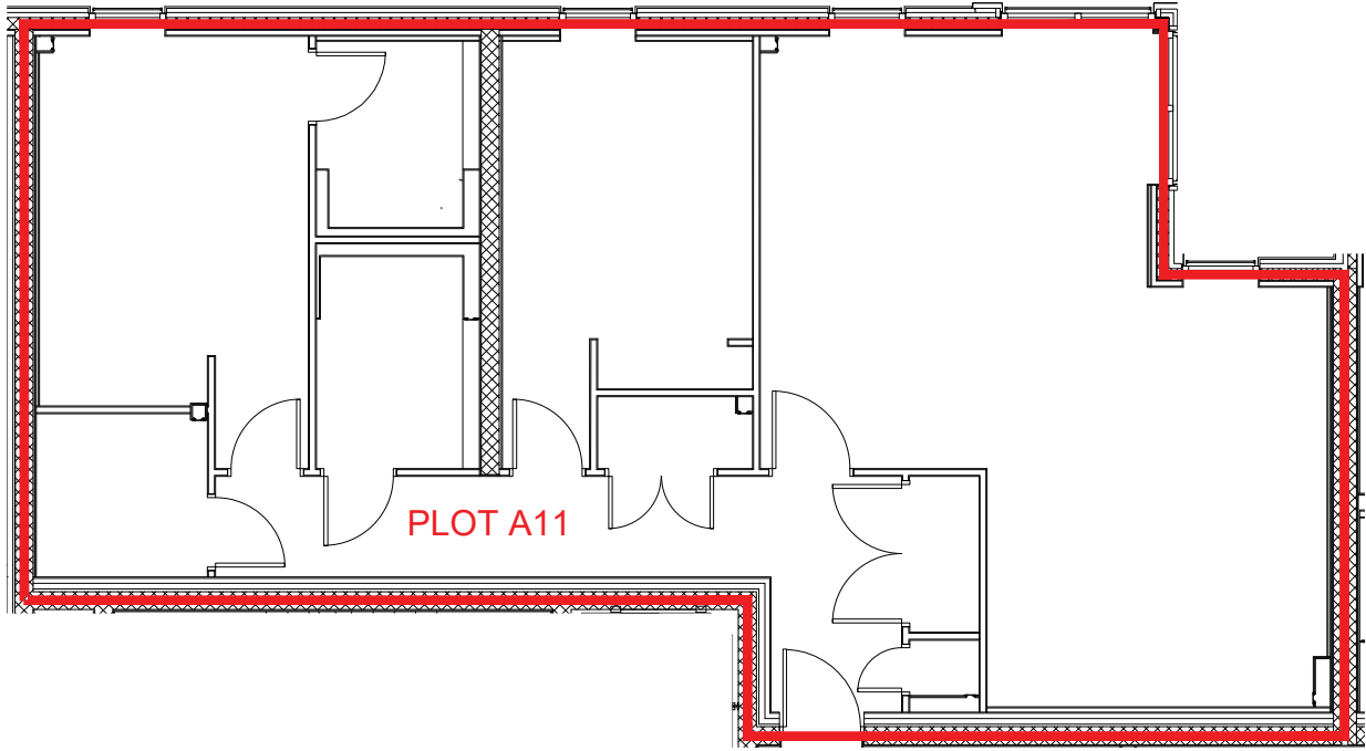
Plot A11 Plan (First Floor) 1:100
