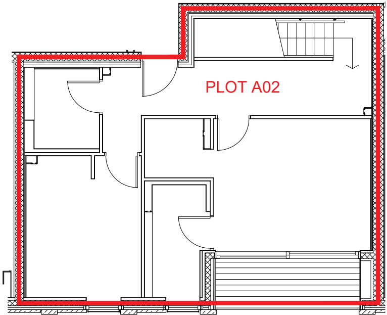
Plot A02 Plan (First Floor) 1:100
