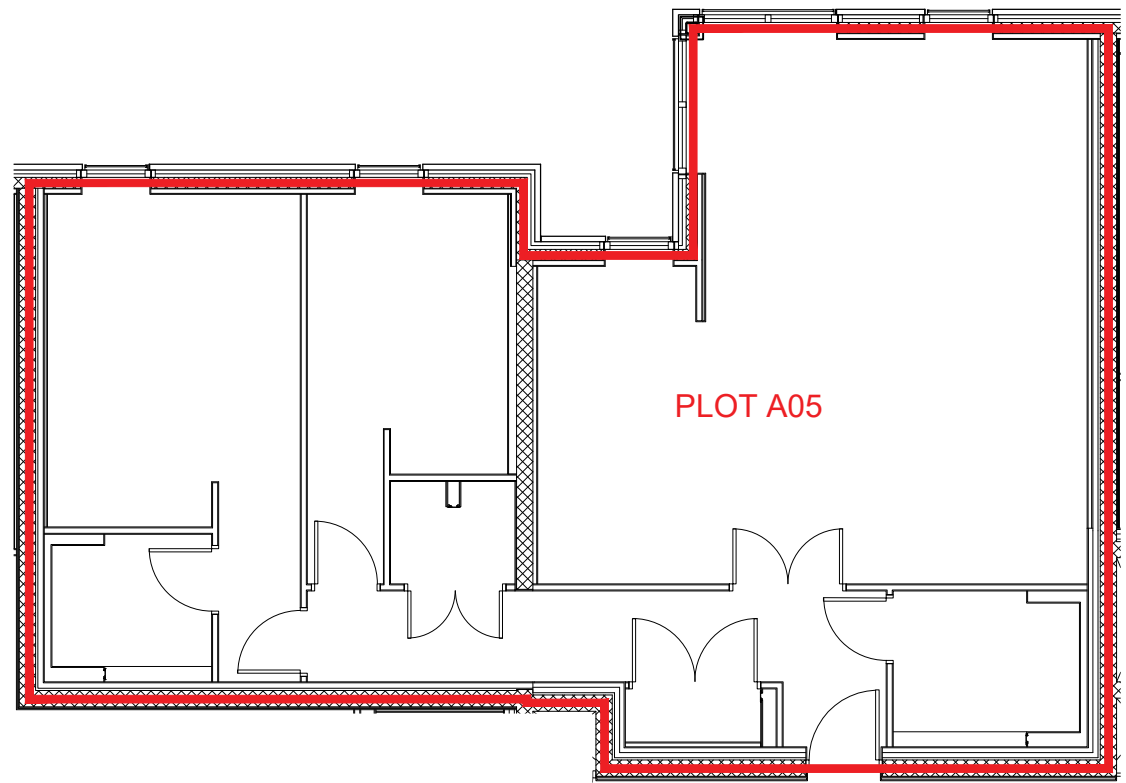
Plot A05 Plan (Ground Floor) 1:100
