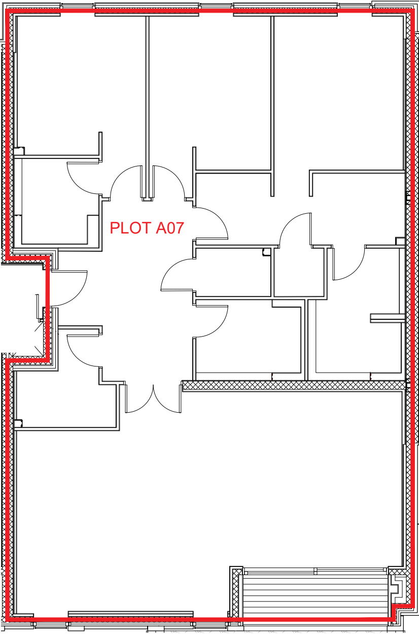
Plot A07 Plan (First Floor) 1:100
