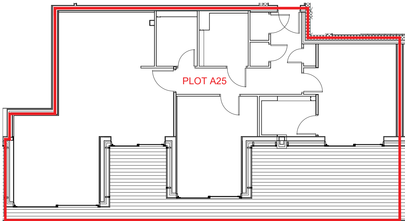
Plot A25 Plan (Fourth Floor) 1:100
