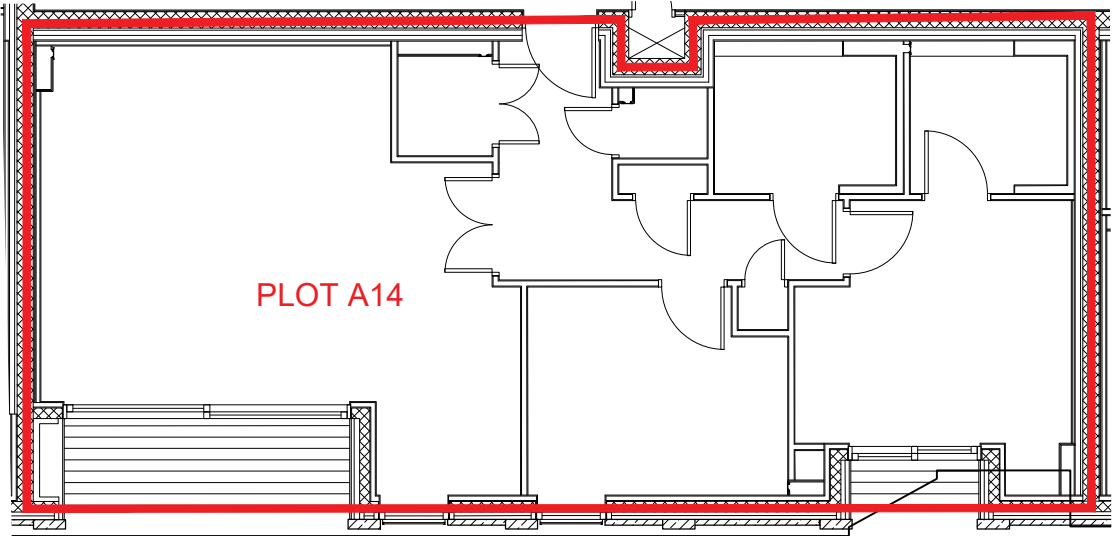
Plot A14 Plan (Second Floor) 1:100
