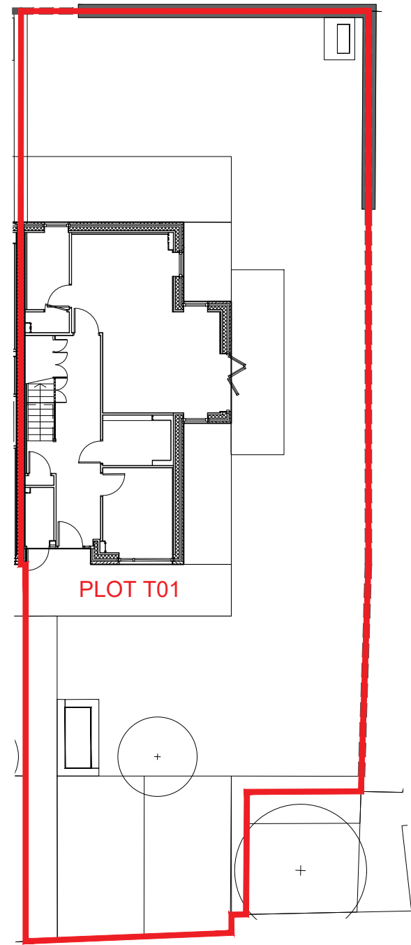
Plot T01 Plan (Ground Floor) 1:200
