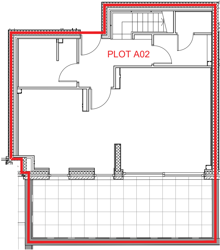
Plot A02 Plan (Ground Floor) 1:100
