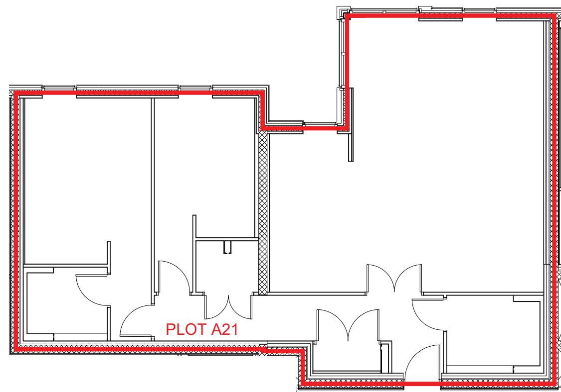
Plot A21 Plan (Third Floor) 1:100
