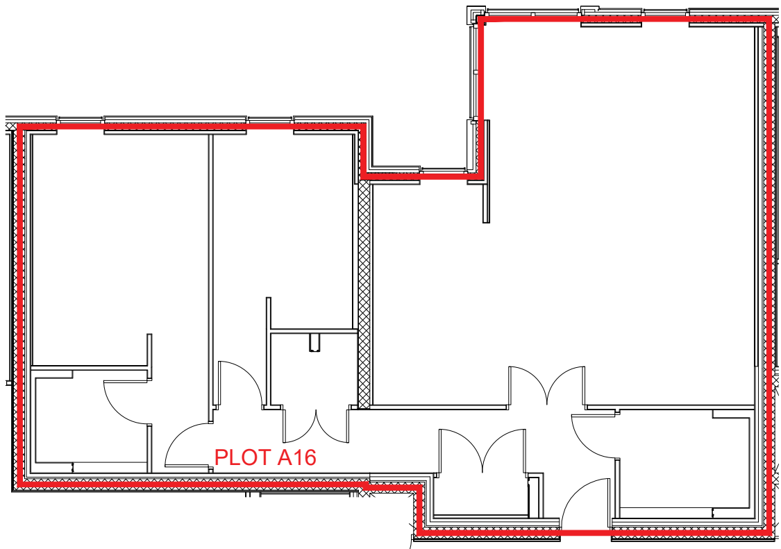
Plot A16 Plan (Second Floor) 1:100
