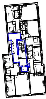
SECOND FLOOR LEVEL
